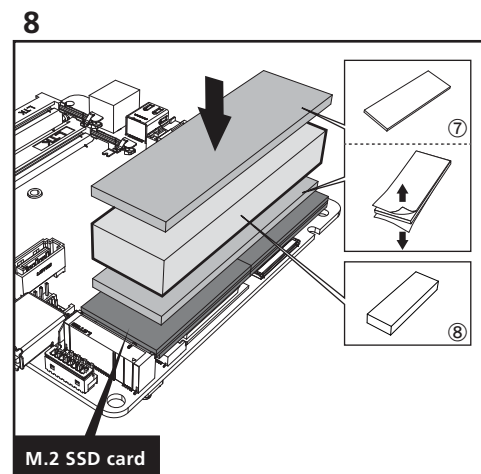
M.2 SSD card
